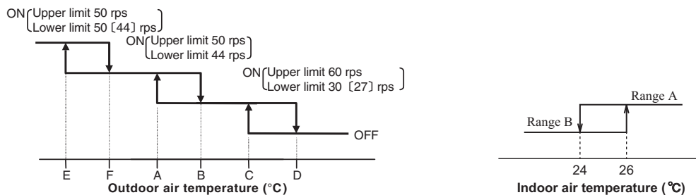
● Values of A, B, C, D, E, F (Models SRK25, 35)
