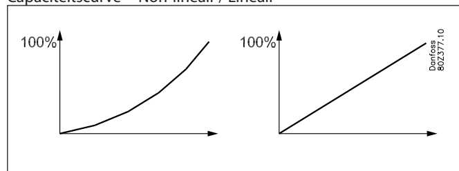
Capaciteitscurve = Non-lineair
